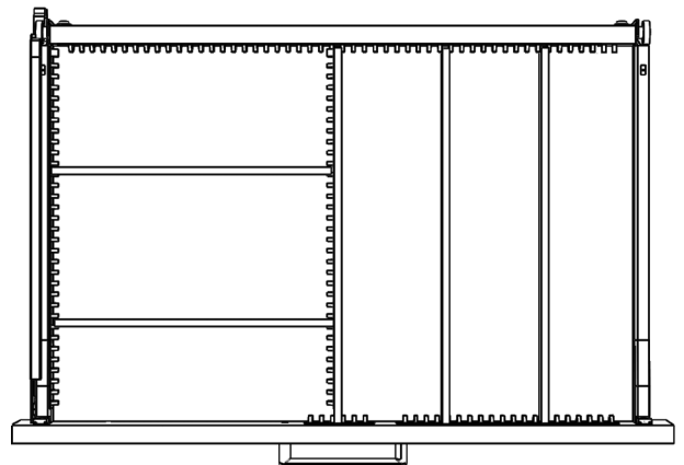
Drawer Divider Combo Kit for One Drawer Part Number S 740282COMB
